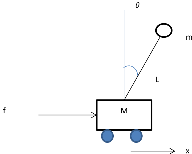
Figure 1: a typical cart-pole system
