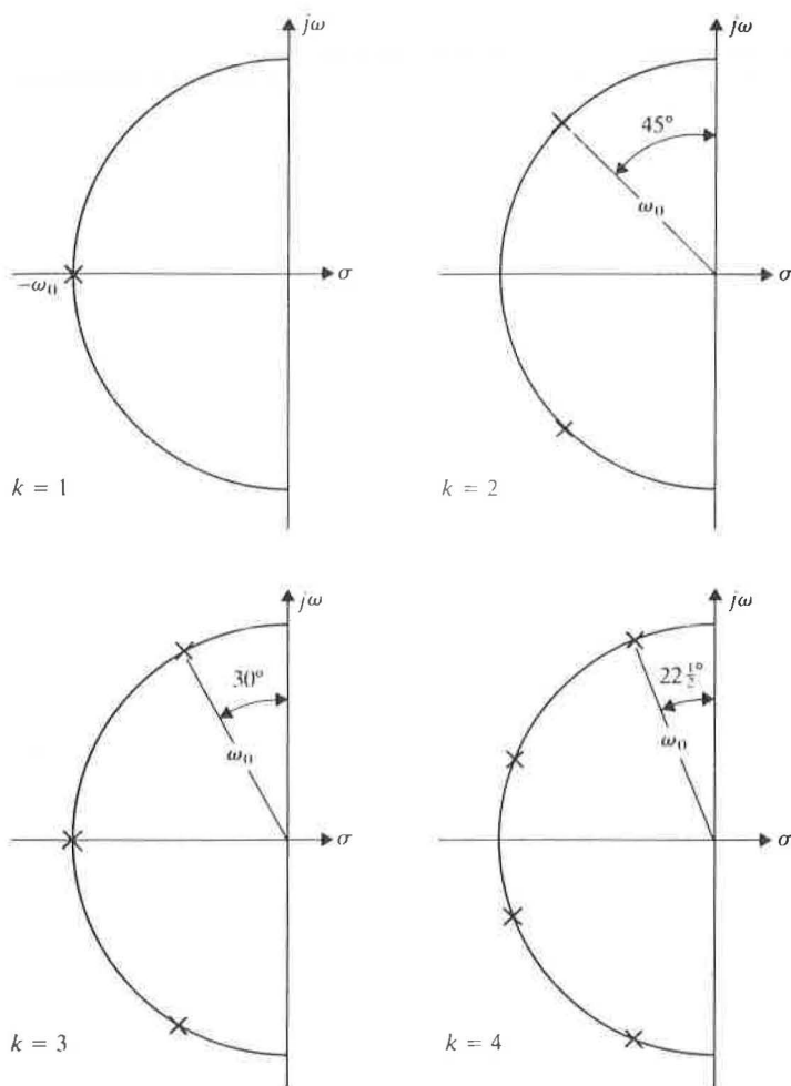
Figure 6.7 Butterworth pole configurations.
