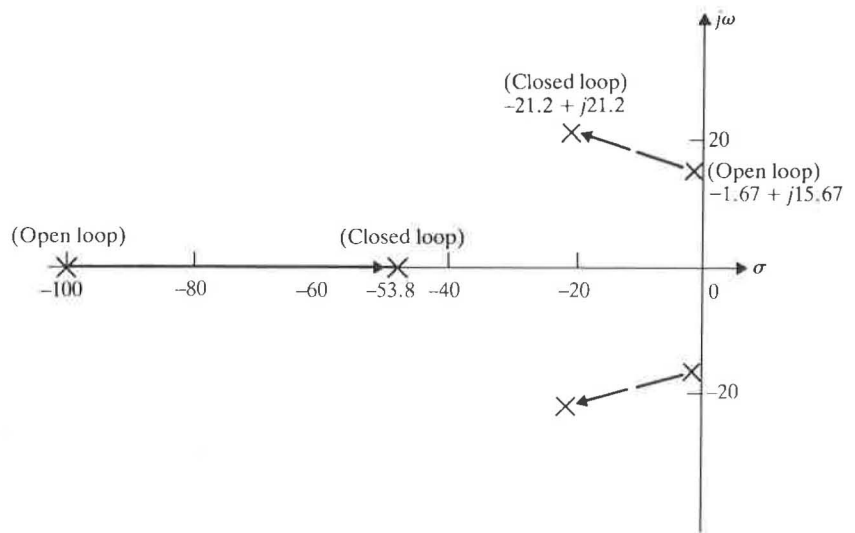
Figure 6.8 Open- and closed-loop poles for missile autopilot.
