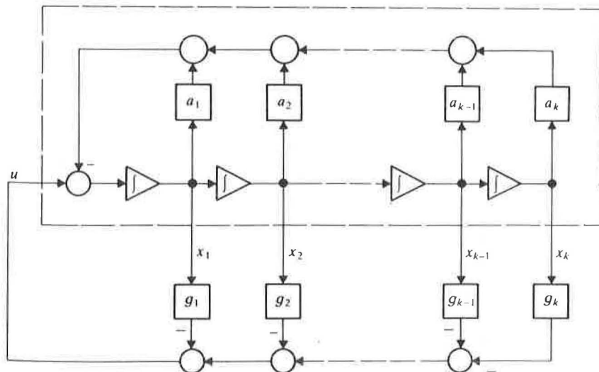
Figure 6.1 State variable feedback for system in first companion form.
