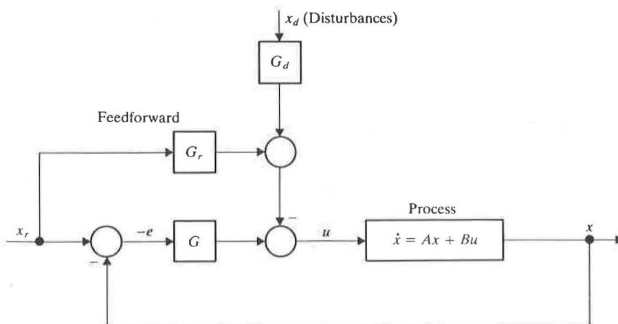
Figure 6.4 Schematic of feedback system for process with reference state and disturbance input.
