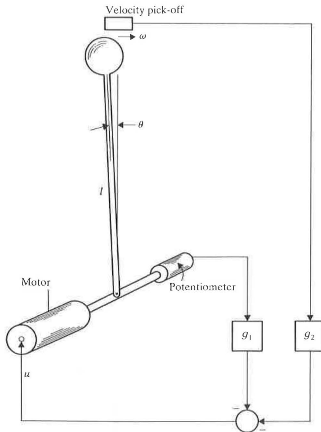
Figure 6.3 Implementation of system to stabilize inverted pendulum.
