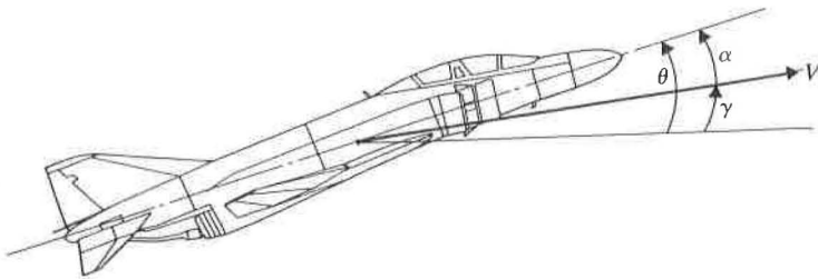
Figure P6.6 Aircraft longitudinal dynamics.
