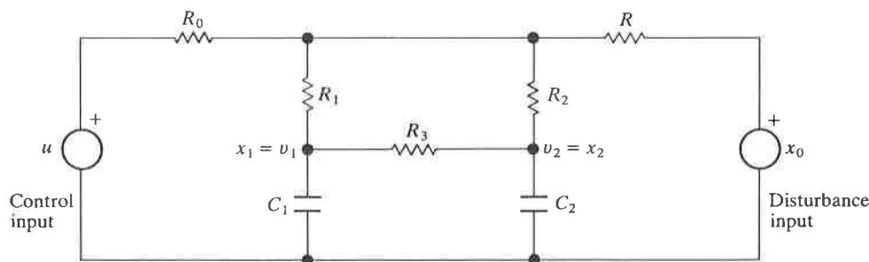
Figure 6.5 Electric network analog of temperature control problem.
