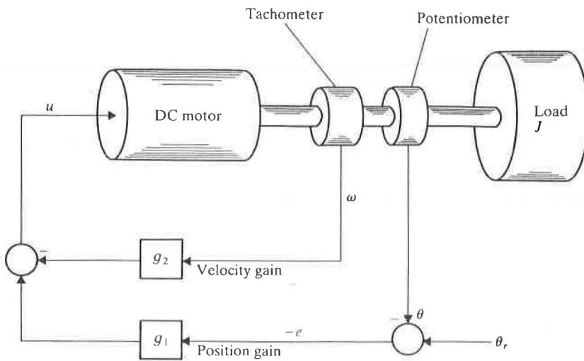
Figure 6.2 Implementation of an instrument servo.
