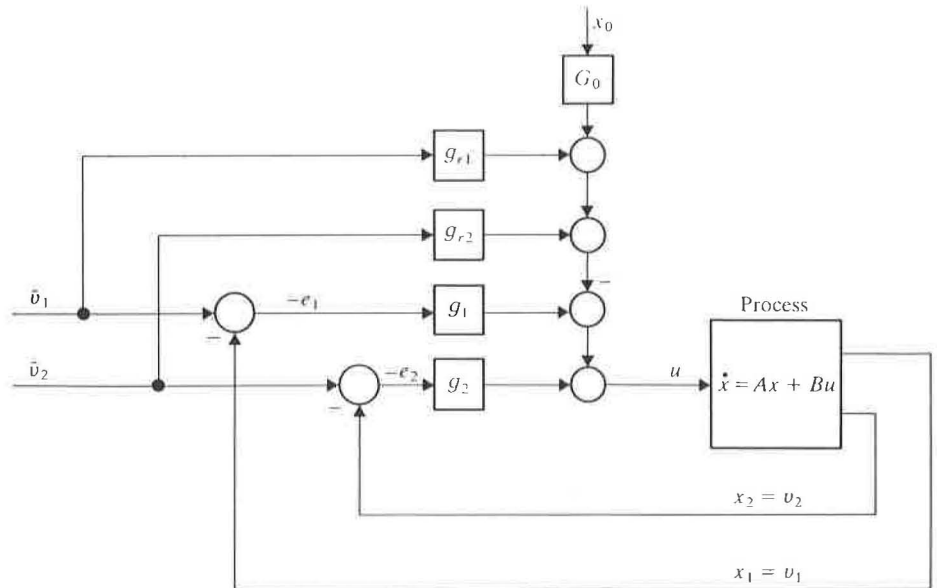
Figure 6.6 Control law implementation.
