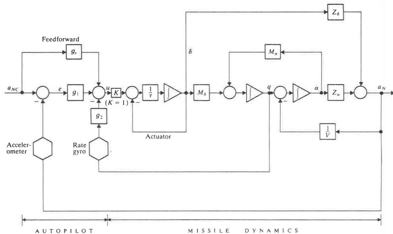
Figure 6.9 Dynamics of missile with autopilot.
